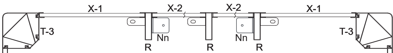
TOP VIEW
