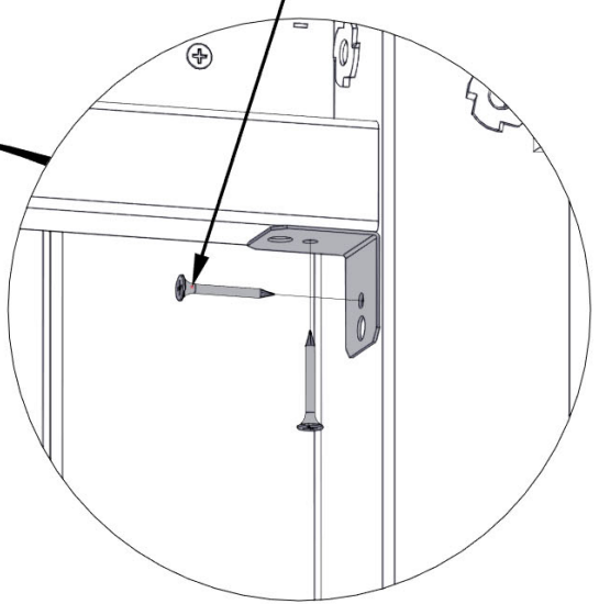
387 (x4) SCREW - 1 1/4"
