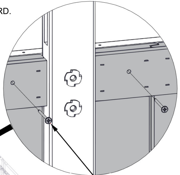
382 (x36) SCREW - 1 3/4"
