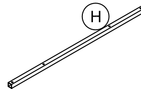
Cross Brace 02 T943360 X 2
