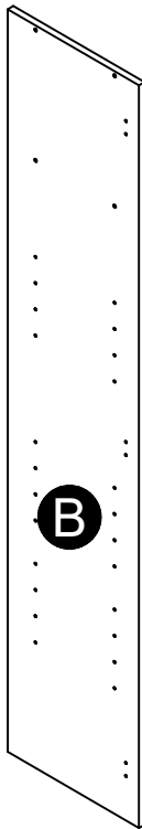
Right Panel 37360015023
