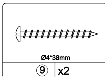
SCREW TDM0010
