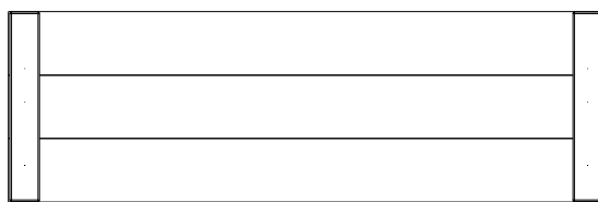
RP6 | W2A03270 - ROOF PANEL (4) | 1 5/8"x15 5/8"x59" (42x396x1204)
