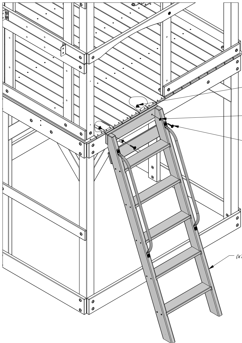
379 (x2) T-NUT - 5/16"
