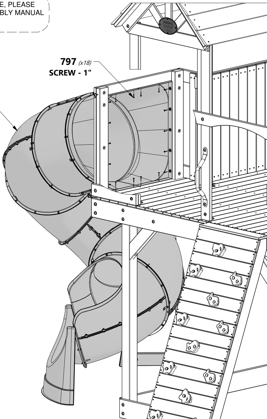
(1) TUBE SLIDE ASSEMBLY
