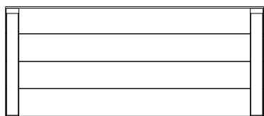
RP3 | ROOF PANEL - W2A03267 (1) | 1 5/8"x20 5/8"x59" (42x524x1204)
