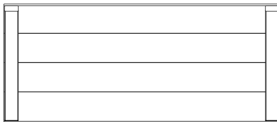
RP3 | ROOF PANEL - W2A03267 (2) | 1 5/8"x20 5/8"x59" (42x524x1204)
