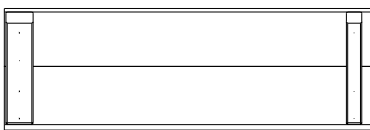
RP1 | ROOF PANEL - W2A03265 (1) | 1 5/8"x10 1/2"x32 7/8" (42x268x812)
