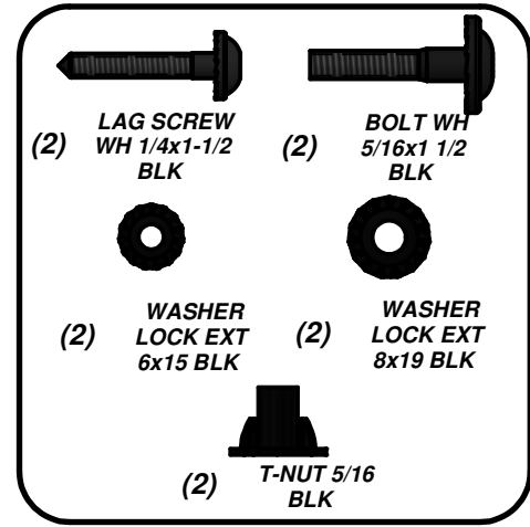
WASHER LOCK EXT 8x19 BLK (2 PLCS)
