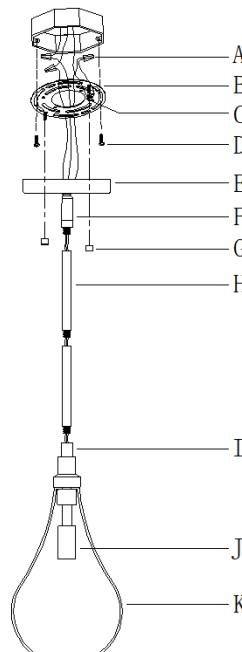
OUTLET BOX
