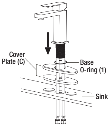
3-Hole Sink Installation
