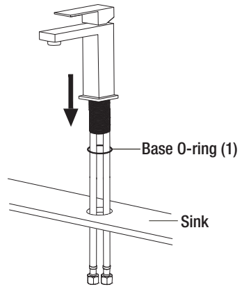
1-Hole Sink Installation
