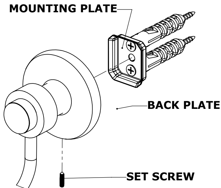
DETAIL N
