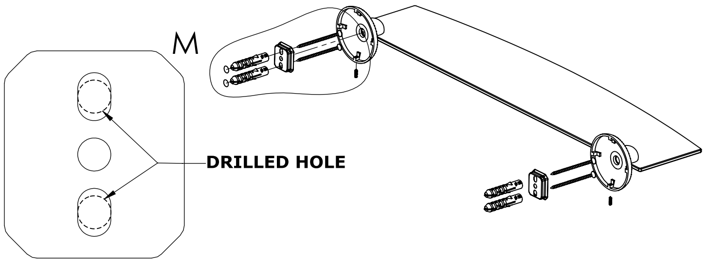
PERSPECTIVE
