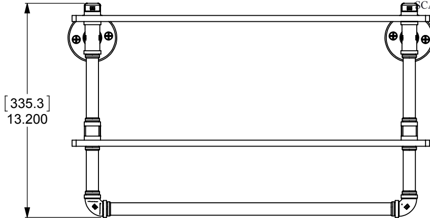
DETAIL AA SCALE 1:2
