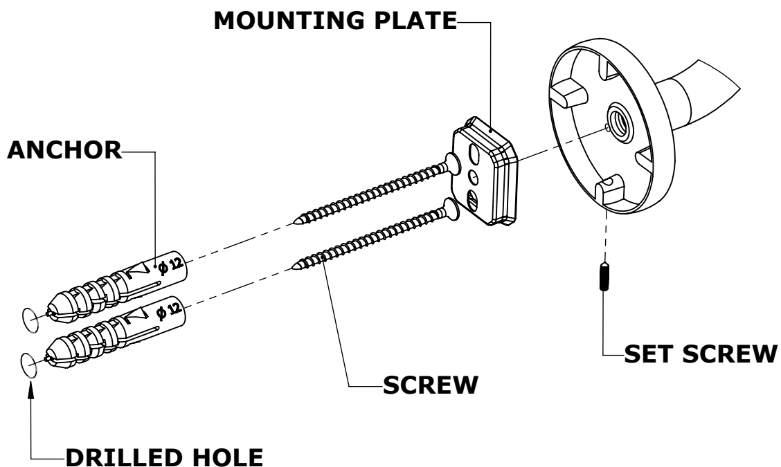
DETAIL M
