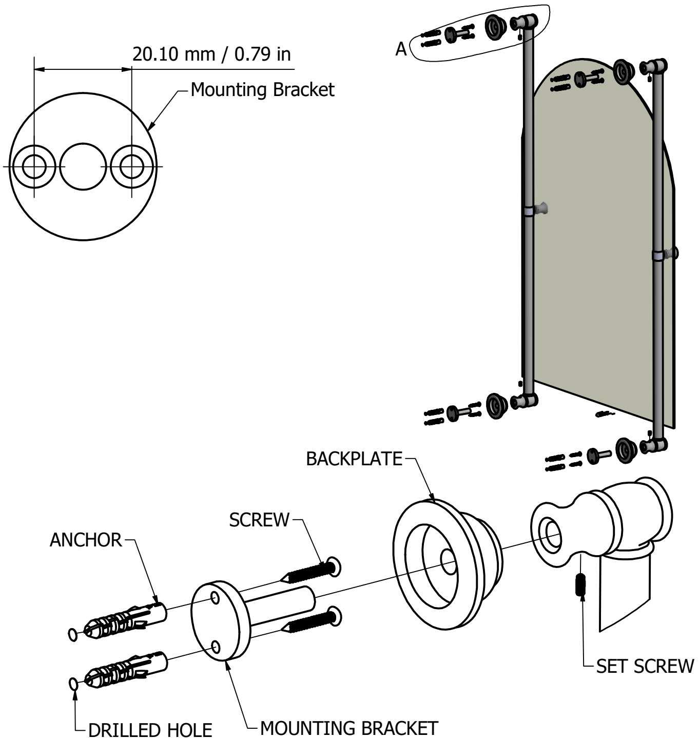
DETAIL A
