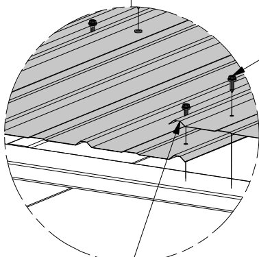
833 (x40) SCREW - 3/4"
