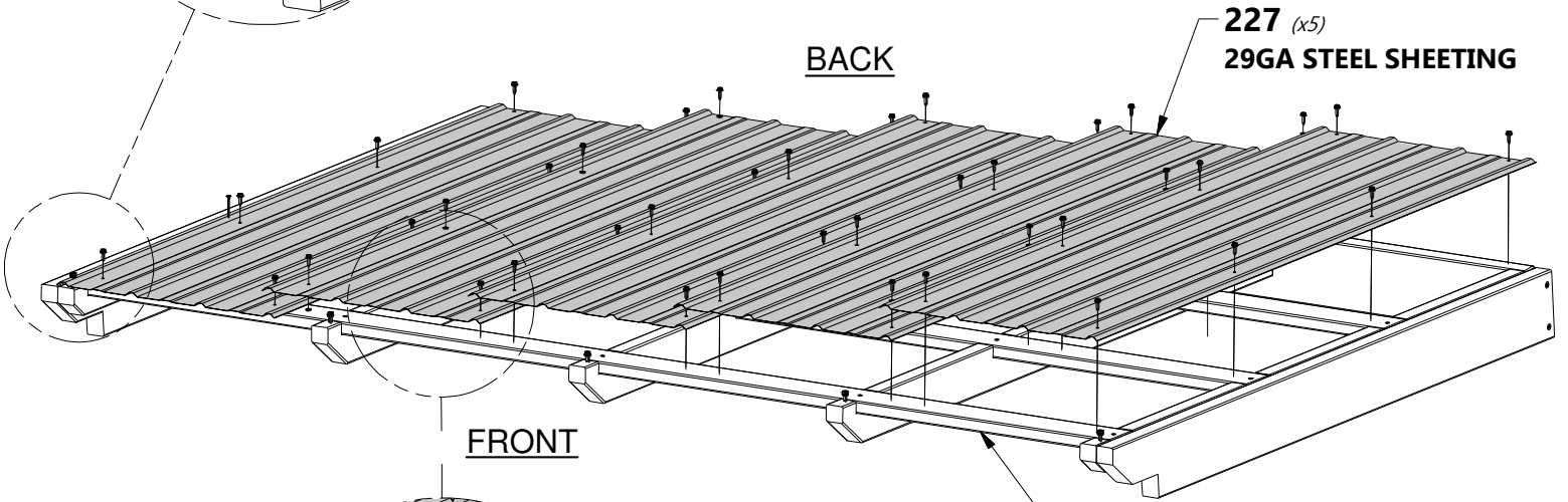
833 (x40) SCREW - 3/4"
