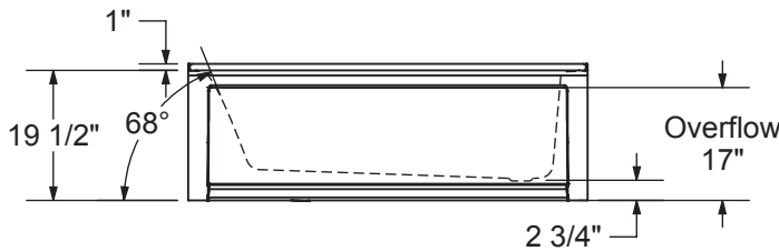
1" Single Integrated tiling flange (shown)
