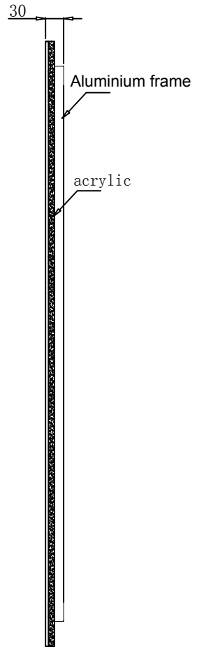
Side View
