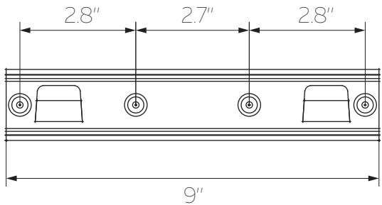
LOWER BRACKET
