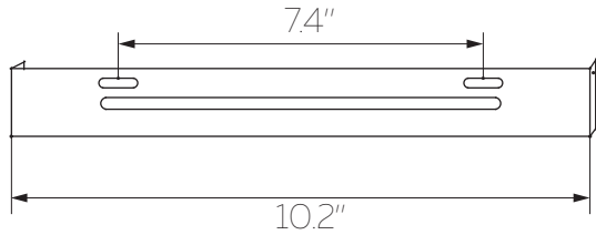
UPPER BRACKET
