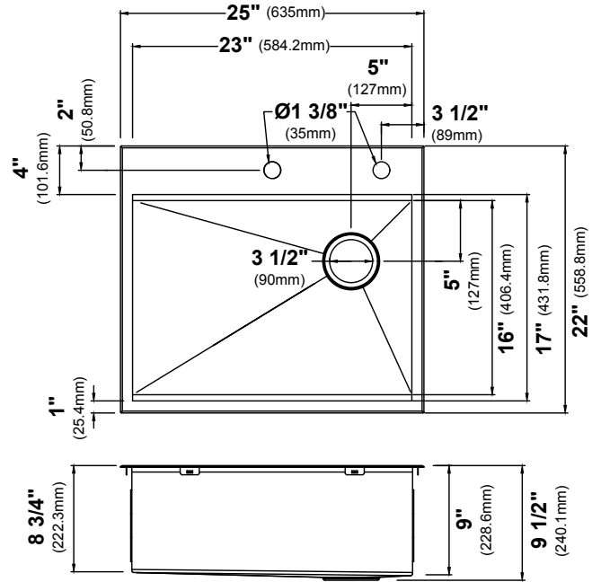
Model #: KWT311-25 Sink Dimensions: 25" x 22" x 9" Min Cabinet Size: 27"
