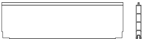
16072 - SLATE - ARDOISE - PIZARRA 15072 - ESPRESSO - EXPRESSO - ESPRESSO FLOOR BOARD A - PLANCHE D'ÉTAGE A - TABLERO DE PISO A 19 7/8IN (50.5 CM) - X1
