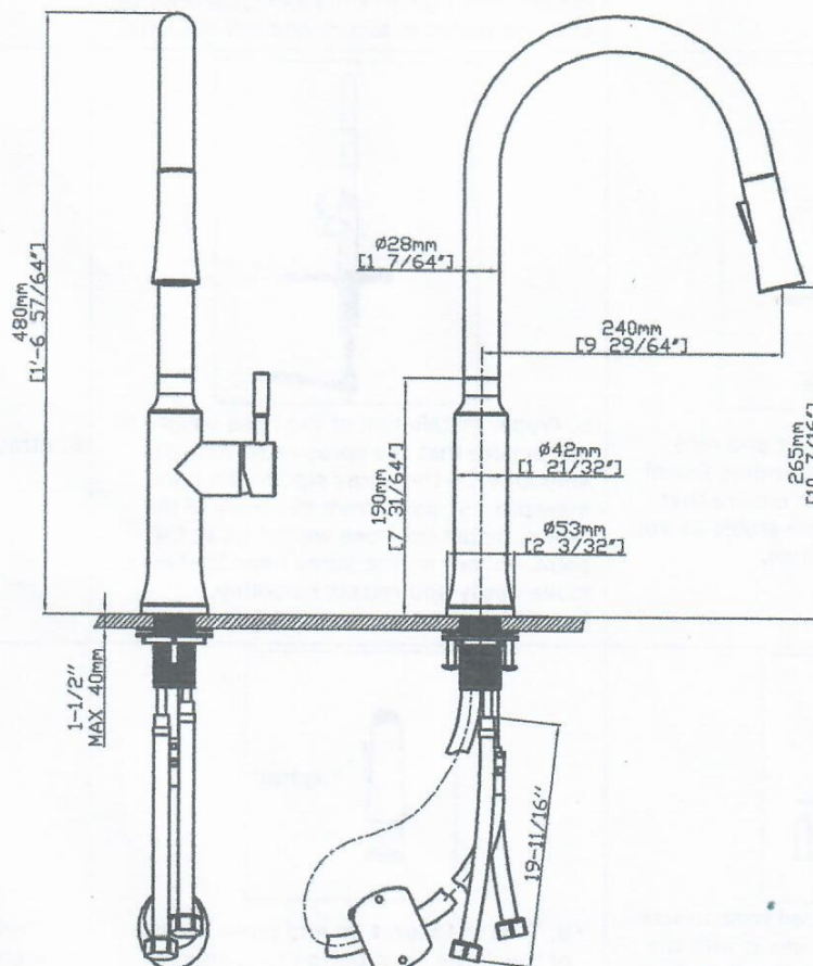
CRITICAL DIMENSIONS
