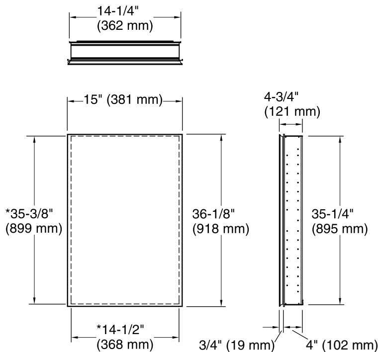
* Recess-Mount Cutout
