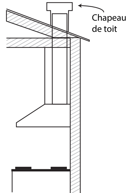
Ventilation murale verticale
