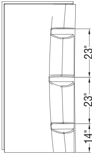
Wall A
