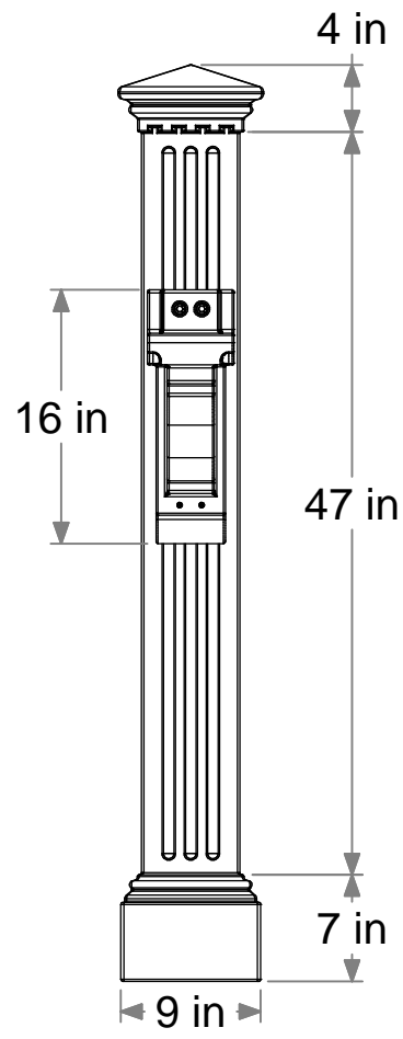
Front View
